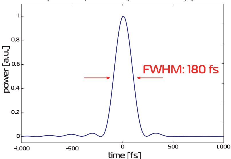
Compressed pulse temporal intensity profile
